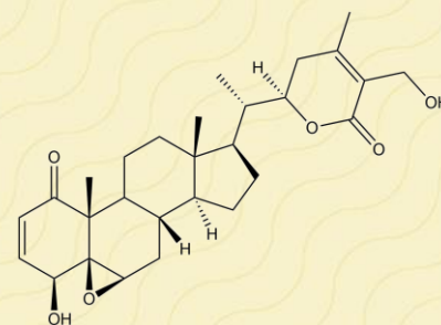
Withaferin A
