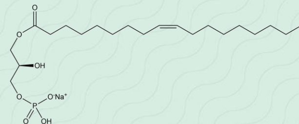
Lysophosphatidic acid
