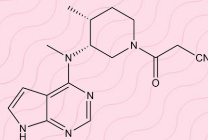
Tofacitinib
